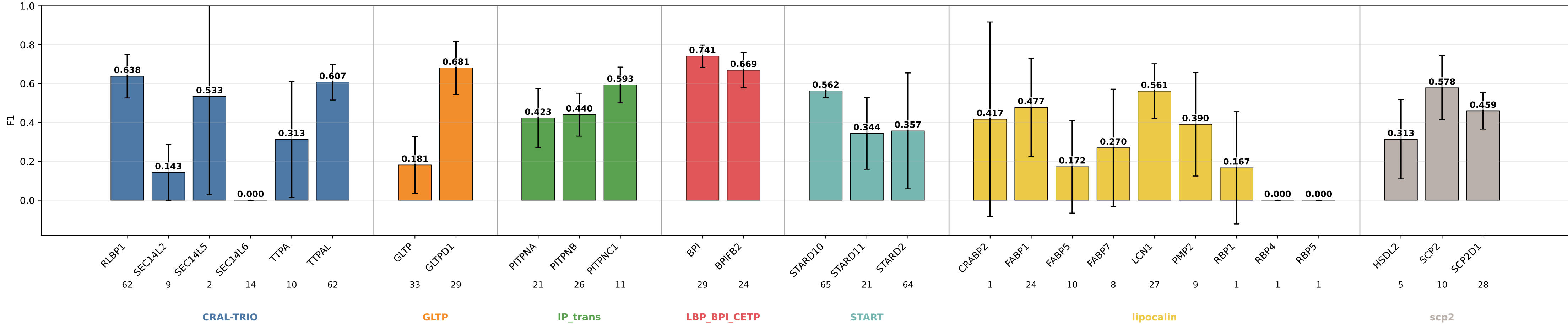
descriptors_1head_coarse F1 by subgroup descriptors_1head_coarse | class weights | lr=0.0001 | weight_decay=0.01 | final_m=4 | final_dropout=0.1 | hiddim=8 | heads=1 | batch=16 | ep=120 | seeds=0,1,2,3,4
