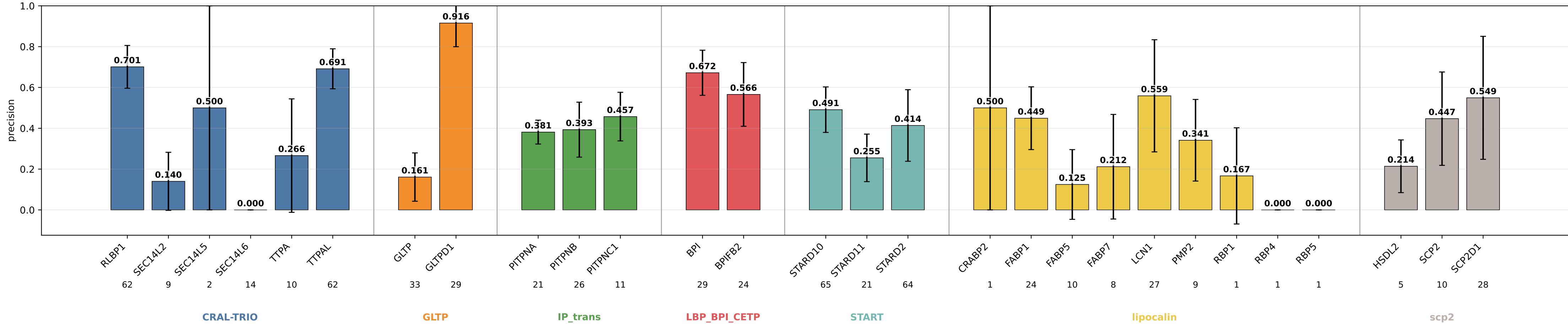
descriptors_1head_coarse precision by subgroup descriptors_1head_coarse | class weights | lr=0.0001 | weight_decay=0.01 | final_m=4 | final_dropout=0.1 | hiddim=8 | heads=1 | batch=16 | ep=120 | seeds=0,1,2,3,4
