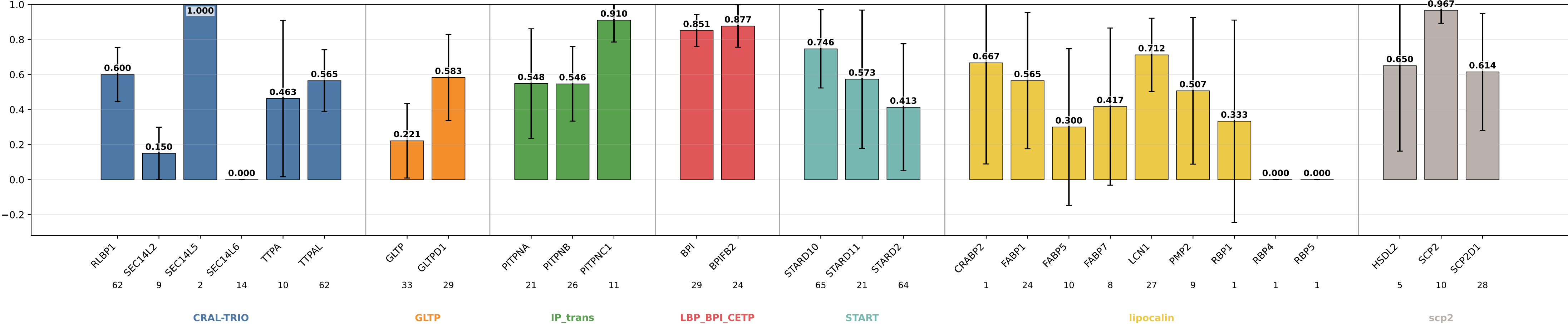
descriptors_1head_coarse sensitivity by subgroup descriptors_1head_coarse | class weights | lr=0.0001 | weight_decay=0.01 | final_m=4 | final_dropout=0.1 | hiddim=8 | heads=1 | batch=16 | ep=120 | seeds=0,1,2,3,4
