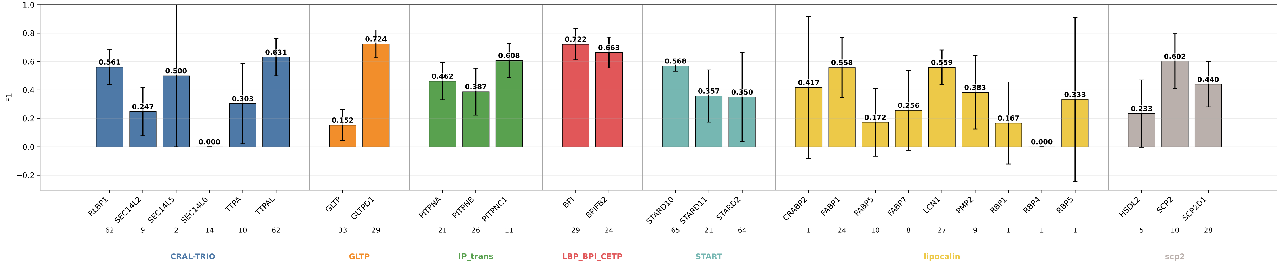
descriptors_2heads_coarse F1 by subgroup descriptors_2heads_coarse | class weights | lr=0.0001 | weight_decay=0.01 | final_m=4 | final_dropout=0.1 | hiddim=8 | heads=2 | batch=16 | ep=120 | seeds=0,1,2,3,4
