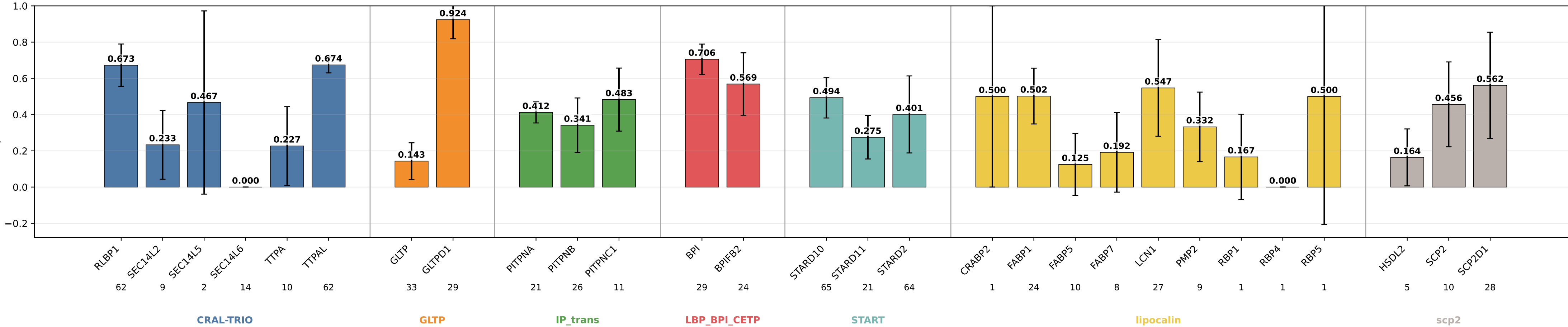
descriptors_2heads_coarse precision by subgroup descriptors_2heads_coarse | class weights | lr=0.0001 | weight_decay=0.01 | final_m=4 | final_dropout=0.1 | hiddim=8 | heads=2 | batch=16 | ep=120 | seeds=0,1,2,3,4
