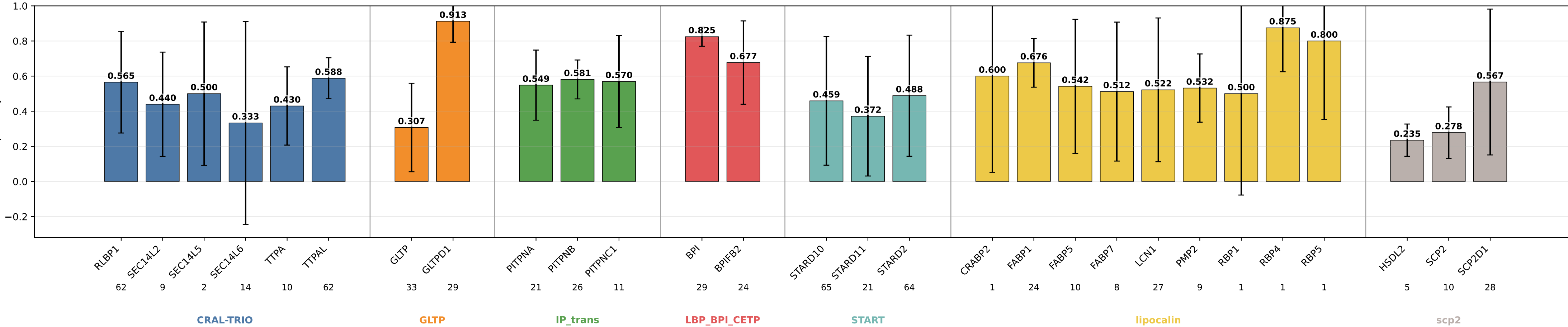
descriptors_2heads_coarse specificity by subgroup descriptors_2heads_coarse | class weights | lr=0.0001 | weight_decay=0.01 | final_m=4 | final_dropout=0.1 | hiddim=8 | heads=2 | batch=16 | ep=120 | seeds=0,1,2,3,4
