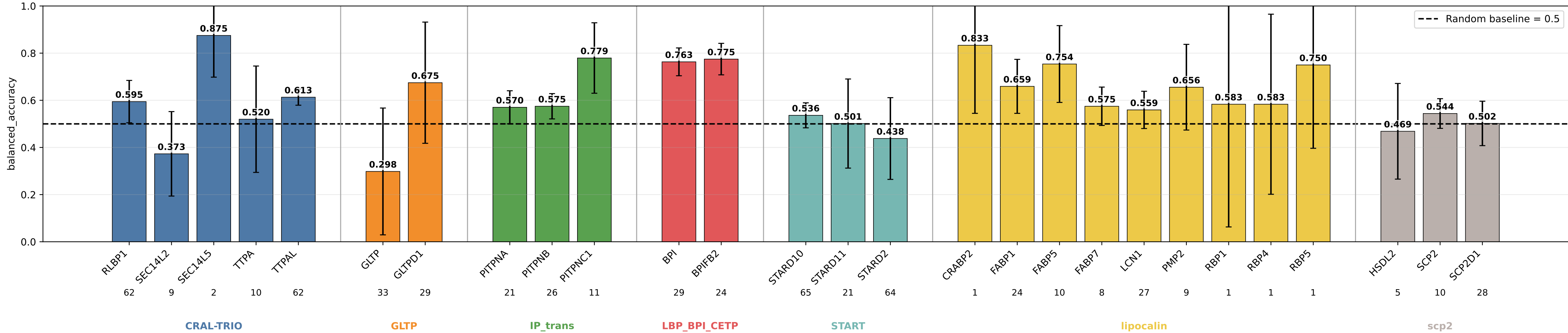
descriptors_3heads_coarse balanced_accuracy by subgroup descriptors_3heads_coarse | class weights | lr=0.0001 | weight_decay=0.01 | final_m=4 | final_dropout=0.1 | hiddim=9 | heads=3 | batch=16 | ep=120 | seeds=0,1,2,3,4
