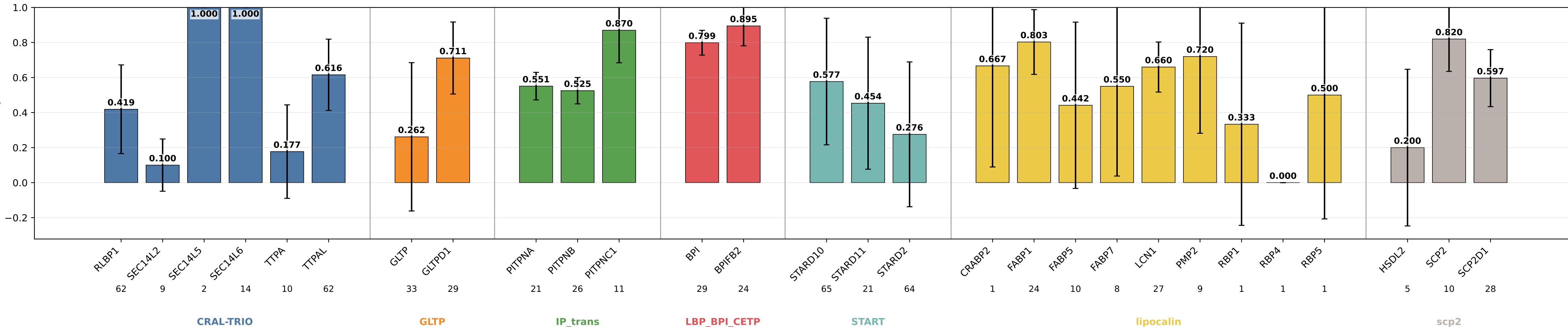
descriptors_No_extent sensitivity by subgroup descriptors_No_extent | class weights | lr=0.0001 | weight_decay=0.01 | final_m=4 | final_dropout=0.1 | hiddim=8 | heads=8 | batch=16 | ep=120 | seeds=0,1,2,3,4
