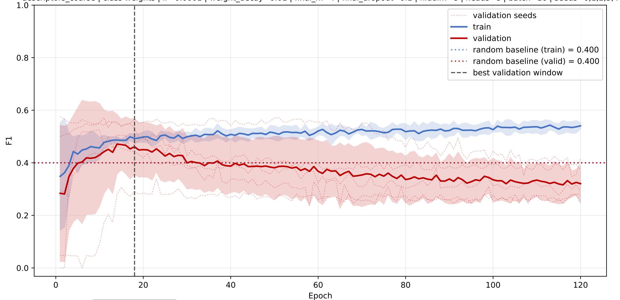
lipocalin: mean F1 learning curve across seeds
