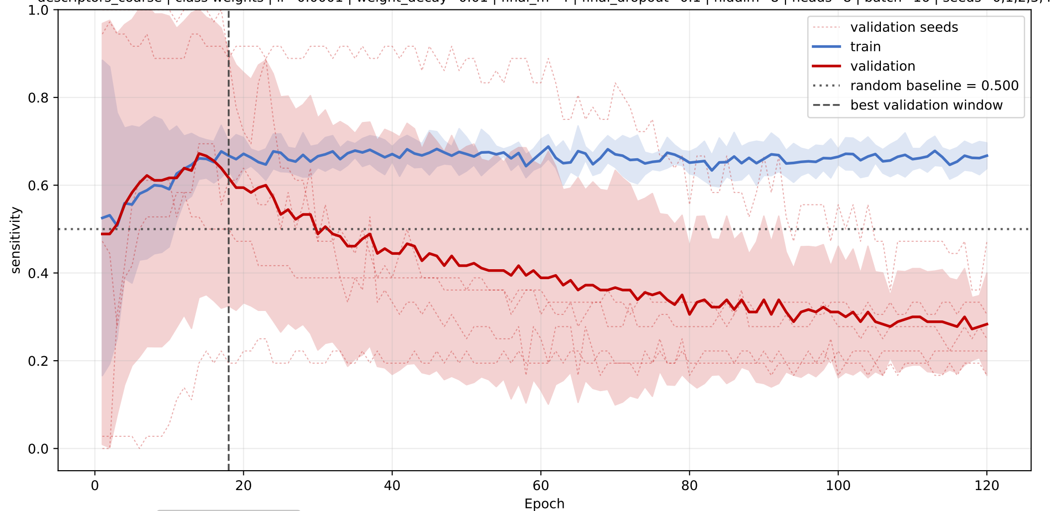
lipocalin: mean sensitivity learning curve across seeds
