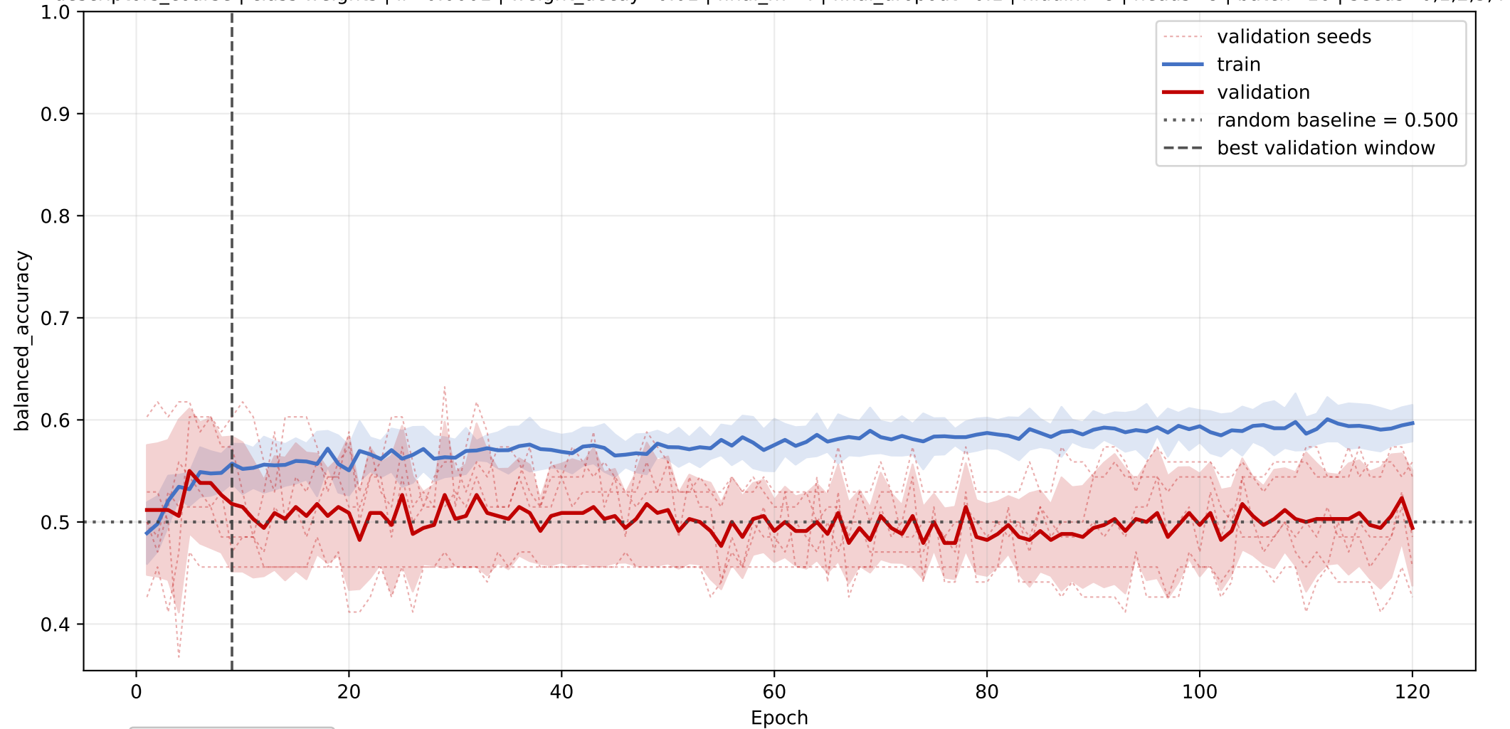
scp2: mean balanced_accuracy learning curve across seeds
