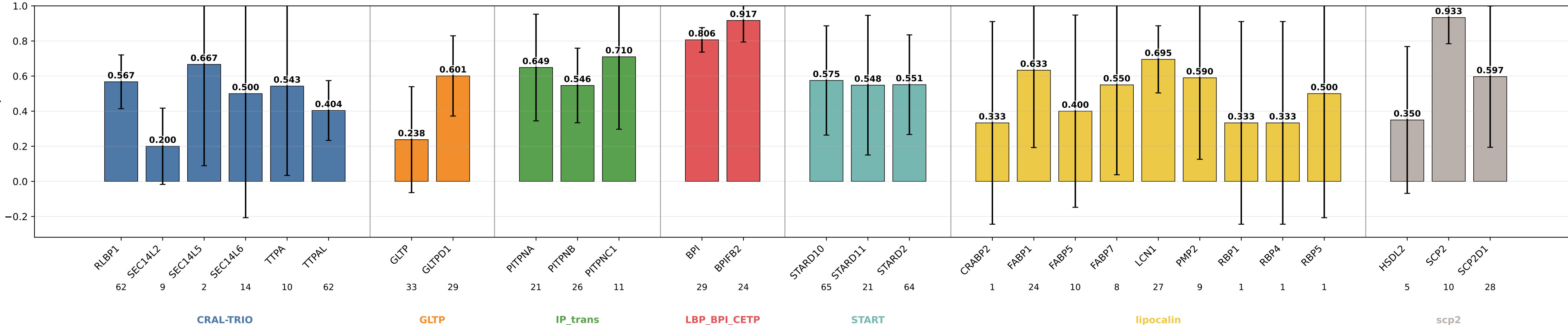
descriptors_coarse sensitivity by subgroup descriptors_coarse | class weights | lr=0.0001 | weight_decay=0.01 | final_m=4 | final_dropout=0.1 | hiddim=8 | heads=8 | batch=16 | ep=120 | seeds=0,1,2,3,4
