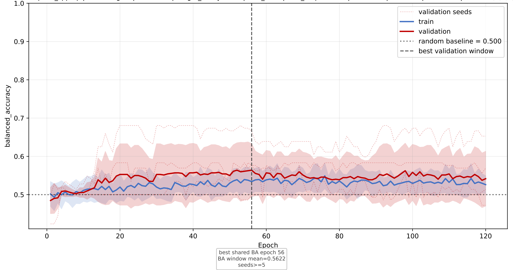
lipocalin: mean balanced_accuracy learning curve across seeds
