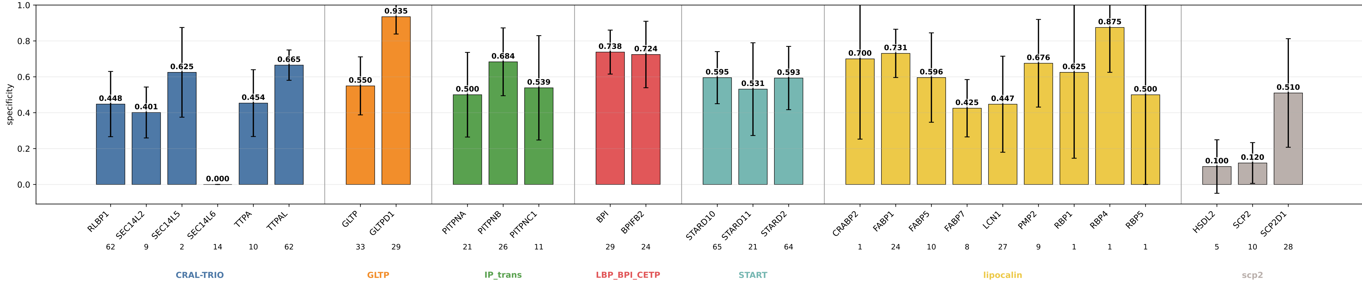
descriptors_mlp_coarse specificity by subgroup descriptors_mlp_coarse | class weights | lr=0.0001 | weight_decay=0.01 | final_m=4 | final_dropout=0.1 | hiddim=8 | heads=8 | batch=16 | ep=120 | seeds=0,1,2,3,4
