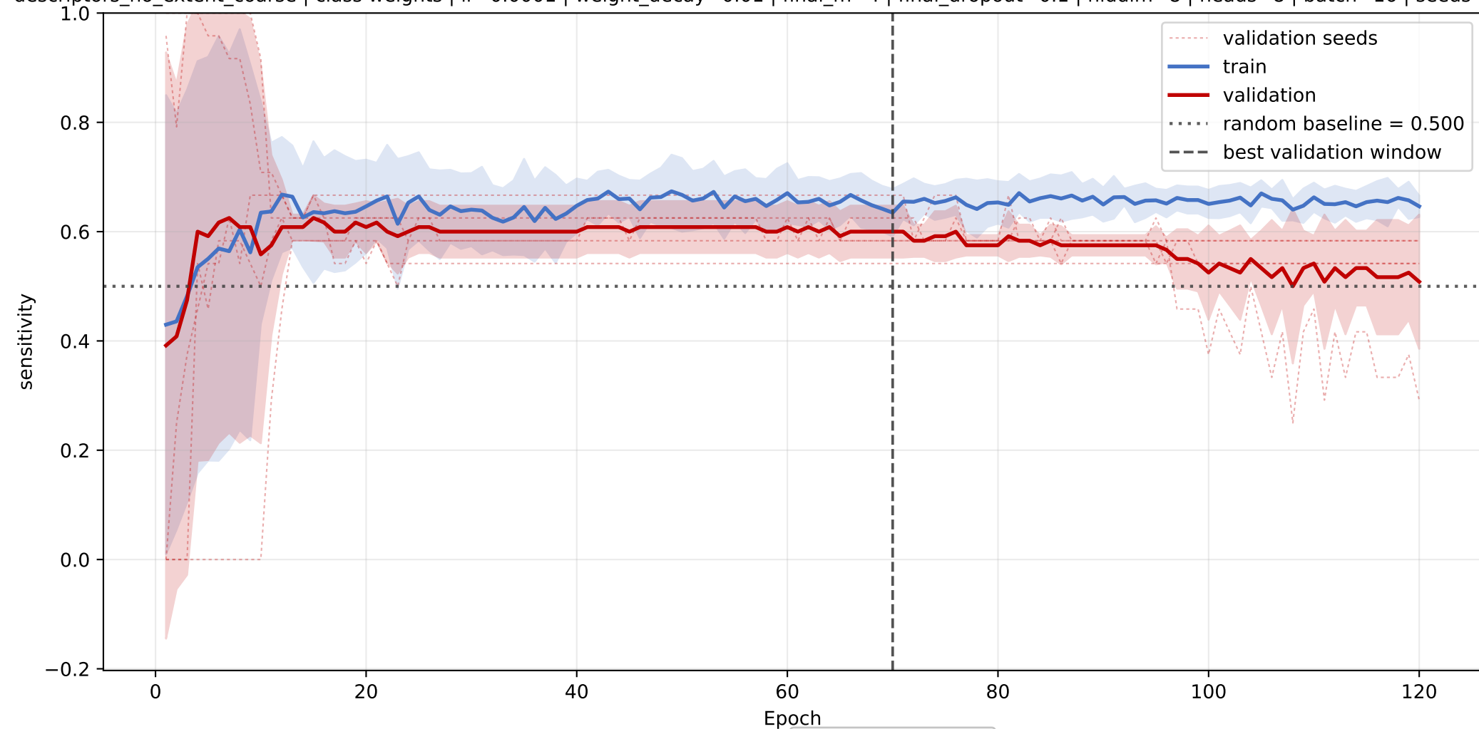
IP_trans: mean sensitivity learning curve across seeds
