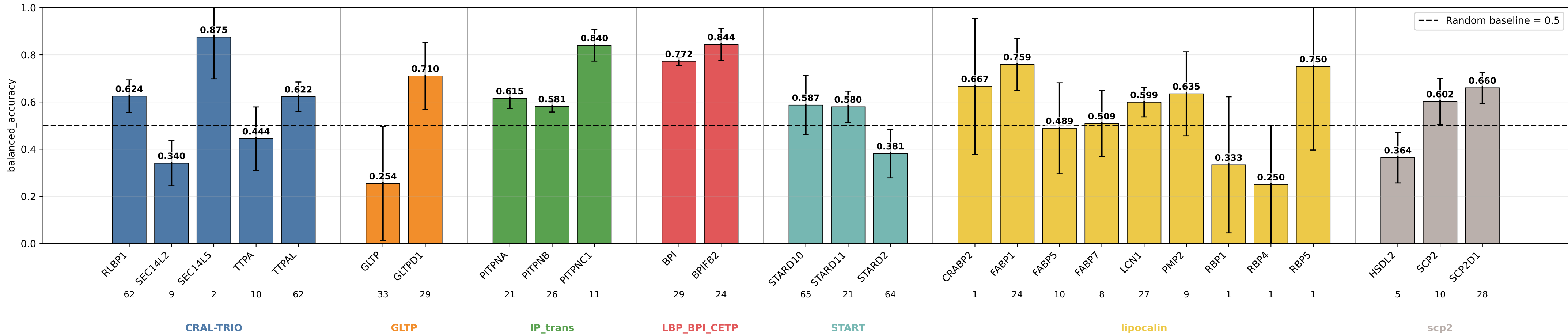
descriptors_no_extent_coarse balanced_accuracy by subgroup descriptors_no_extent_coarse | class weights | lr=0.0001 | weight_decay=0.01 | final_m=4 | final_dropout=0.1 | hiddim=8 | heads=8 | batch=16 | ep=120 | seeds=0,1,2,3,4
