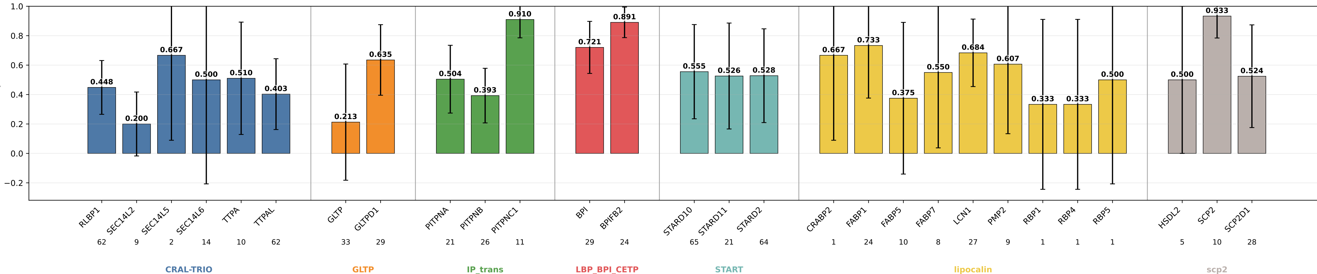
descriptors_no_extent_coarse_add_dpt005 sensitivity by subgroup descriptors_no_extent_coarse_add_dpt005 | class weights | lr=0.0001 | weight_decay=0.01 | final_m=4 | final_dropout=0.005 | hiddim=8 | heads=8 | batch=16 | ep=120 | seeds=0,1,2,3,4
