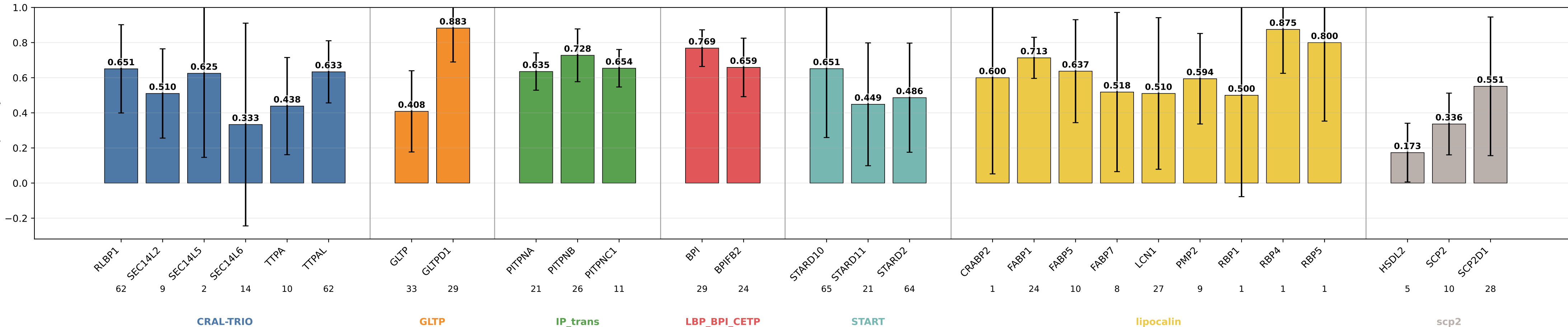
descriptors_no_extent_coarse_add_dpt005 specificity by subgroup descriptors_no_extent_coarse_add_dpt005 | class weights | lr=0.0001 | weight_decay=0.01 | final_m=4 | final_dropout=0.005 | hiddim=8 | heads=8 | batch=16 | ep=120 | seeds=0,1,2,3,4
