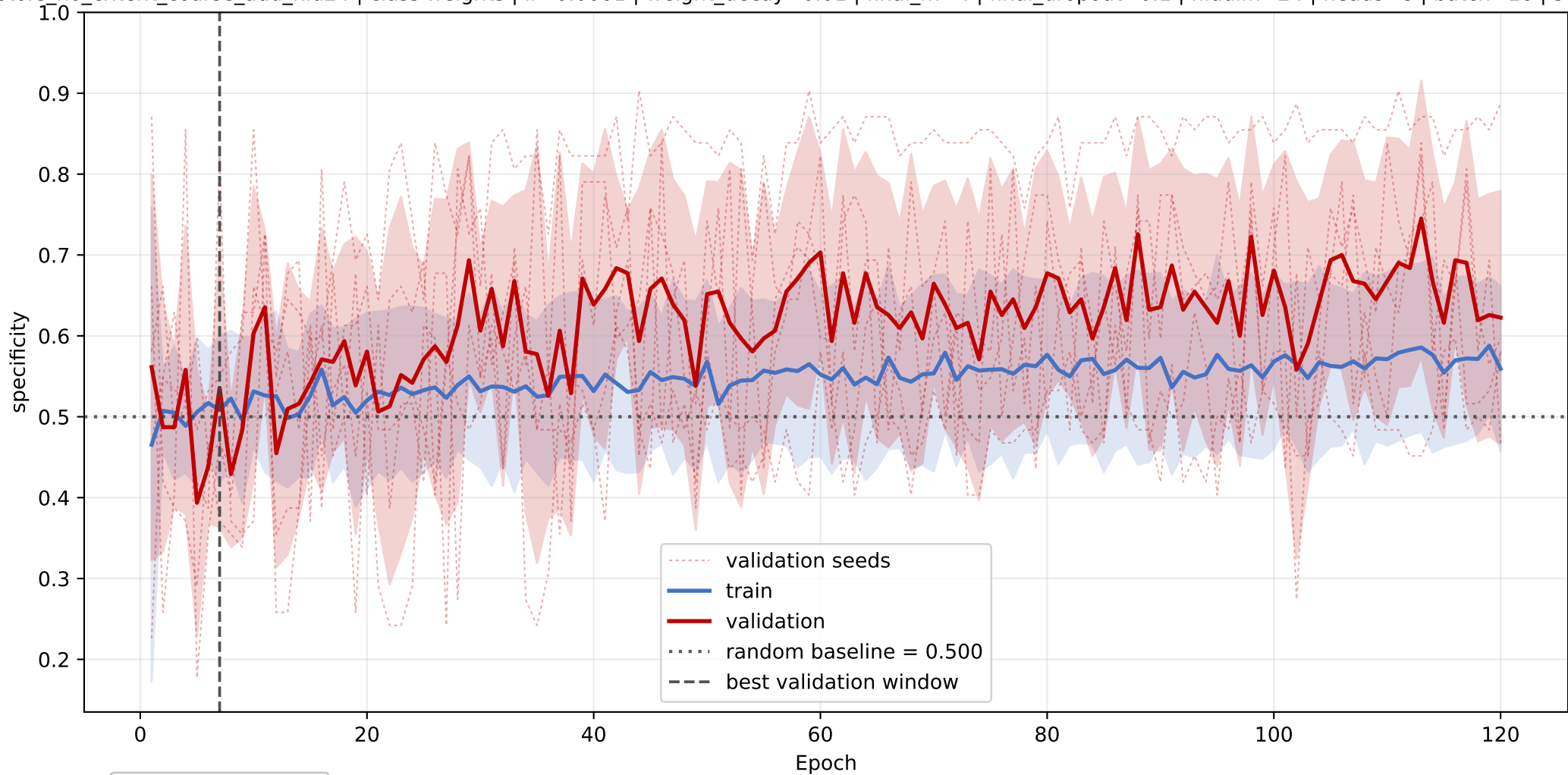
CRAL-TRIO: mean specificity learning curve across seeds
