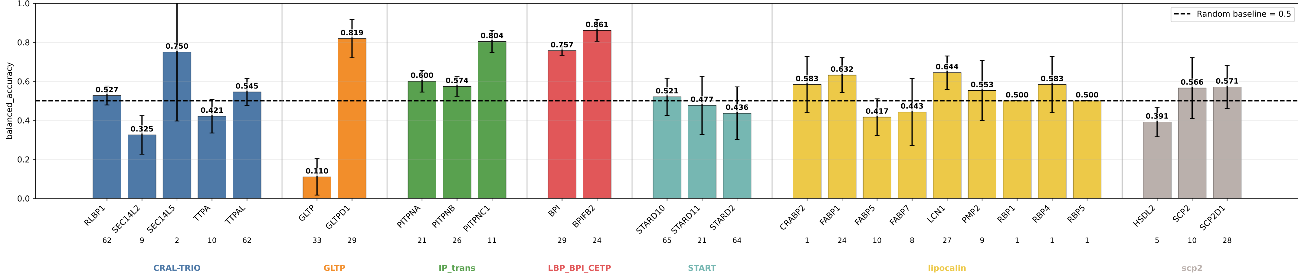
descriptors_no_extent_coarse_add_hid24 balanced_accuracy by subgroup descriptors_no_extent_coarse_add_hid24 | class weights | lr=0.0001 | weight_decay=0.01 | final_m=4 | final_dropout=0.1 | hiddim=24 | heads=8 | batch=16 | ep=120 | seeds=0,1,2,3,4
