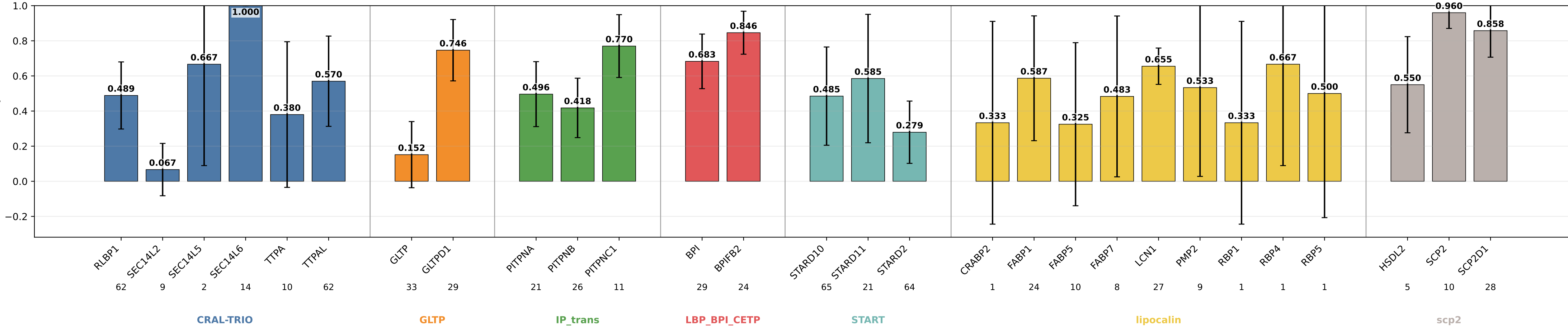
descriptors_no_extent_coarse_add_hid32 sensitivity by subgroup descriptors_no_extent_coarse_add_hid32 | class weights | lr=0.0001 | weight_decay=0.01 | final_m=4 | final_dropout=0.1 | hiddim=32 | heads=8 | batch=16 | ep=120 | seeds=0,1,2,3,4
