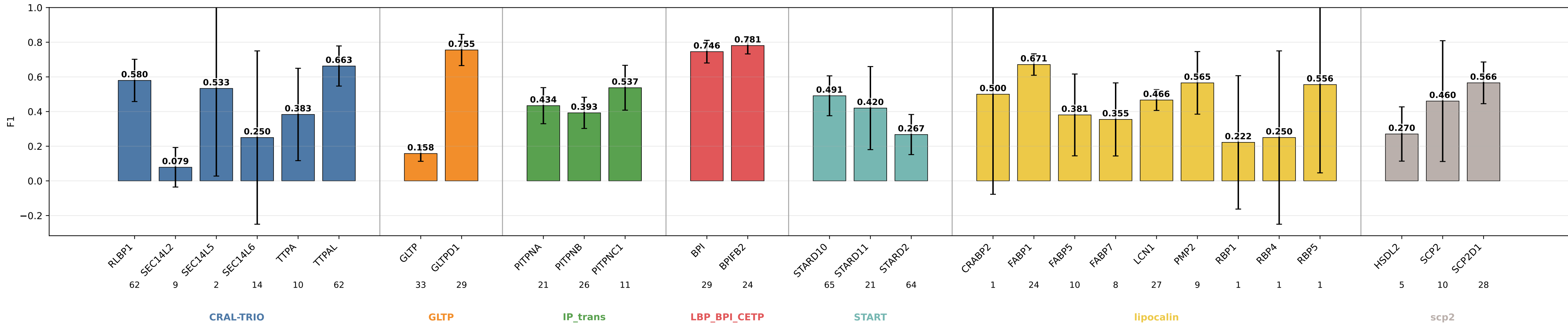
descriptors_no_extent_coarse_add_lipprop F1 by subgroup descriptors_no_extent_coarse_add_lipprop | class weights | lr=0.0001 | weight_decay=0.01 | final_m=4 | final_dropout=0.1 | hiddim=8 | heads=8 | batch=16 | ep=120 | seeds=0,1,2,3,4
