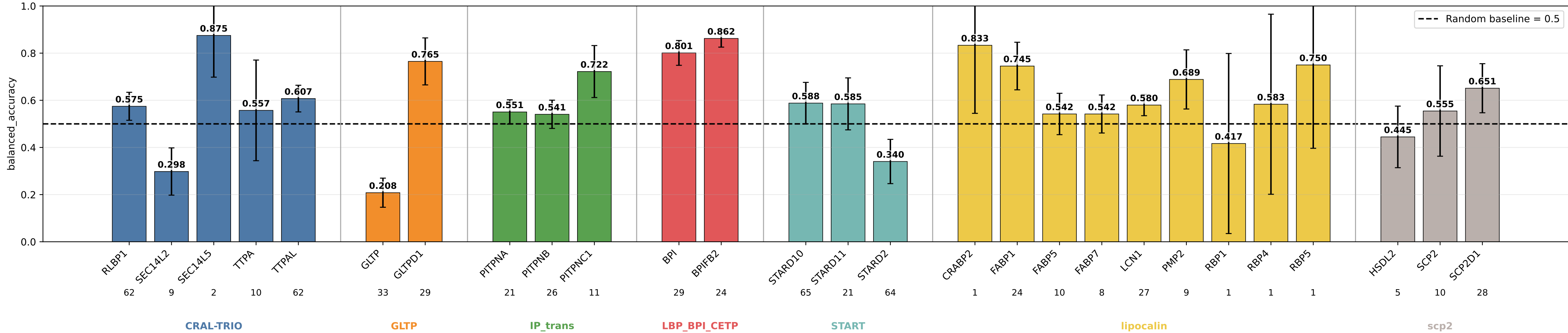
descriptors_no_extent_coarse_add_lipprop balanced_accuracy by subgroup descriptors_no_extent_coarse_add_lipprop | class weights | lr=0.0001 | weight_decay=0.01 | final_m=4 | final_dropout=0.1 | hiddim=8 | heads=8 | batch=16 | ep=120 | seeds=0,1,2,3,4
