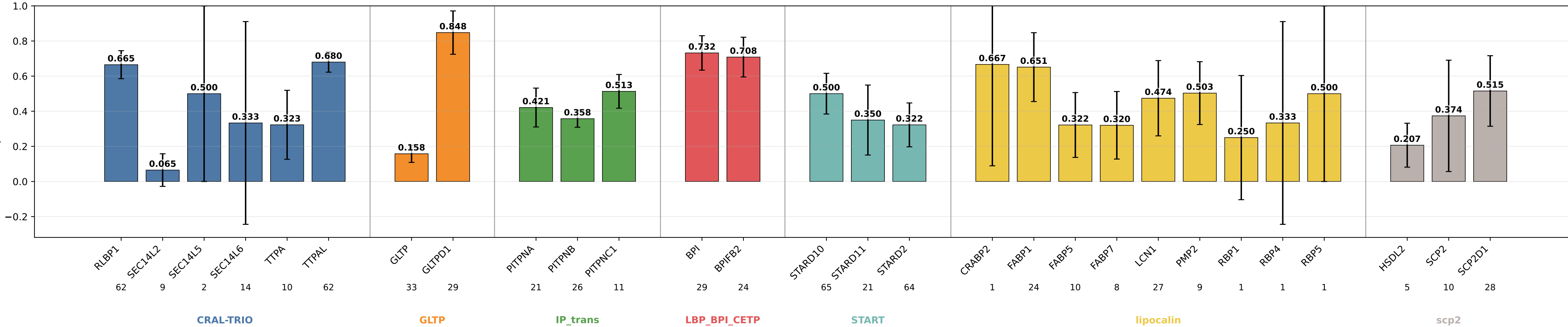
descriptors_no_extent_coarse_add_lipprop precision by subgroup descriptors_no_extent_coarse_add_lipprop | class weights | lr=0.0001 | weight_decay=0.01 | final_m=4 | final_dropout=0.1 | hiddim=8 | heads=8 | batch=16 | ep=120 | seeds=0,1,2,3,4
