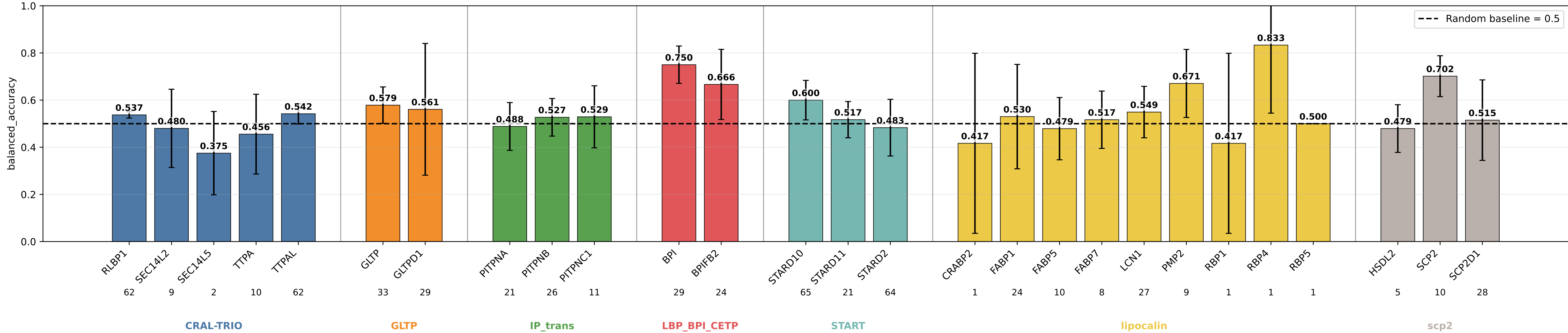
descriptors_no_extent_coarse_add_lipprop_dpt005 balanced_accuracy by subgroup descriptors_no_extent_coarse_add_lipprop_dpt005 | class weights | lr=0.0001 | weight_decay=0.01 | final_m=4 | final_dropout=0.005 | hiddim=8 | heads=8 | batch=16 | ep=120 | seeds=0,1,2,3,4
