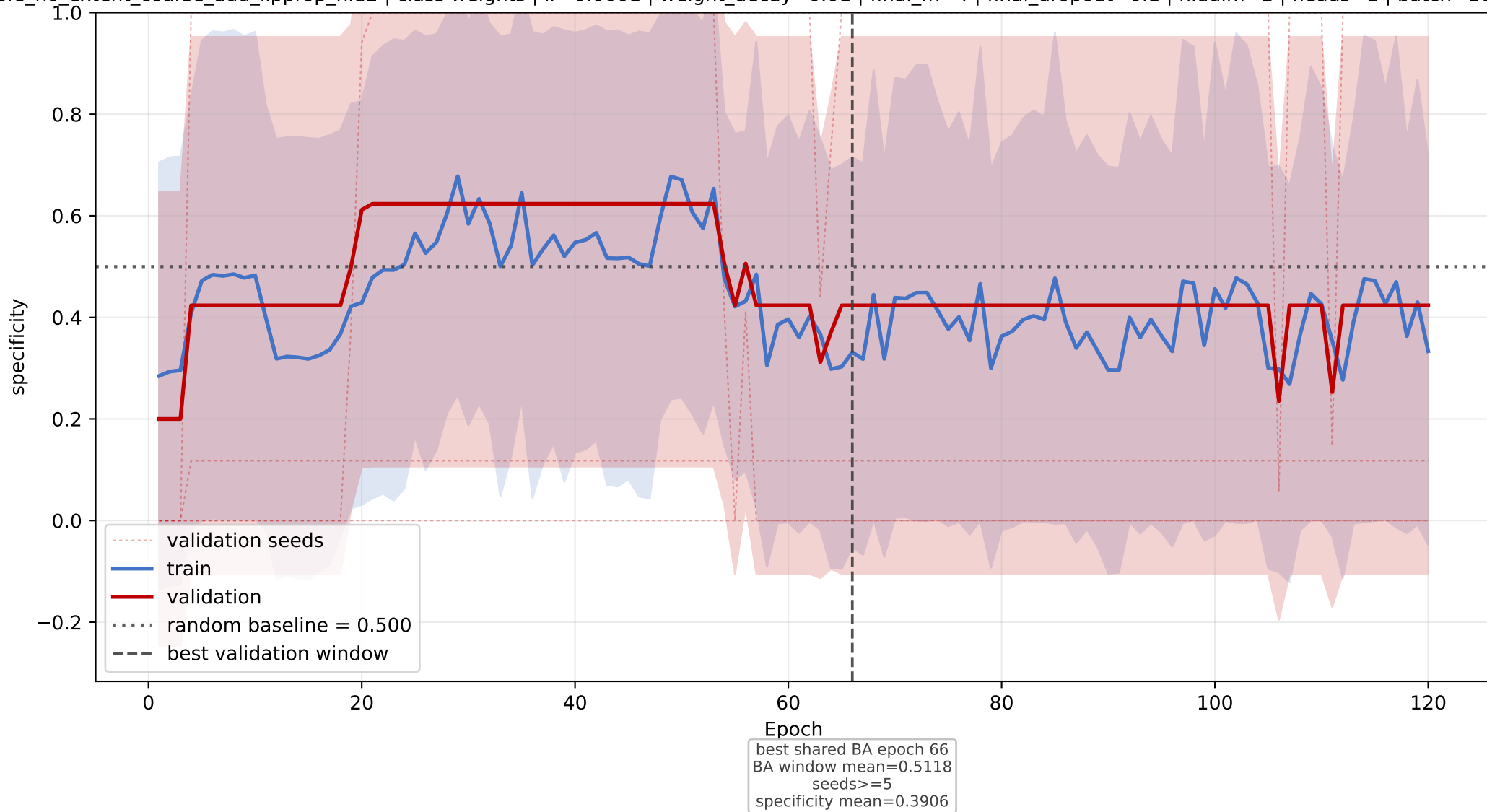
scp2: mean specificity learning curve across seeds
