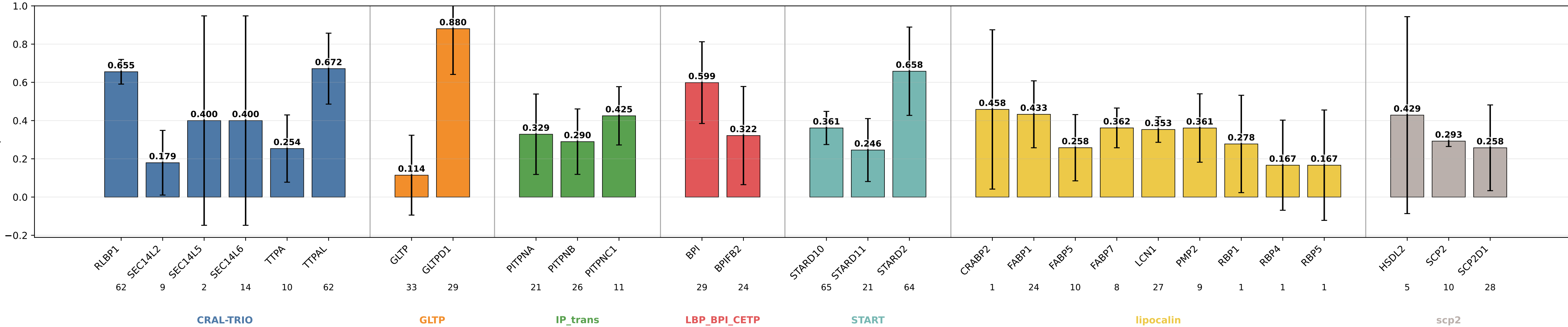
descriptors_no_extent_coarse_add_lipprop_hid2 precision by subgroup descriptors_no_extent_coarse_add_lipprop_hid2 | class weights | lr=0.0001 | weight_decay=0.01 | final_m=4 | final_dropout=0.1 | hiddim=2 | heads=1 | batch=16 | ep=120 | seeds=0,1,2,3,4
