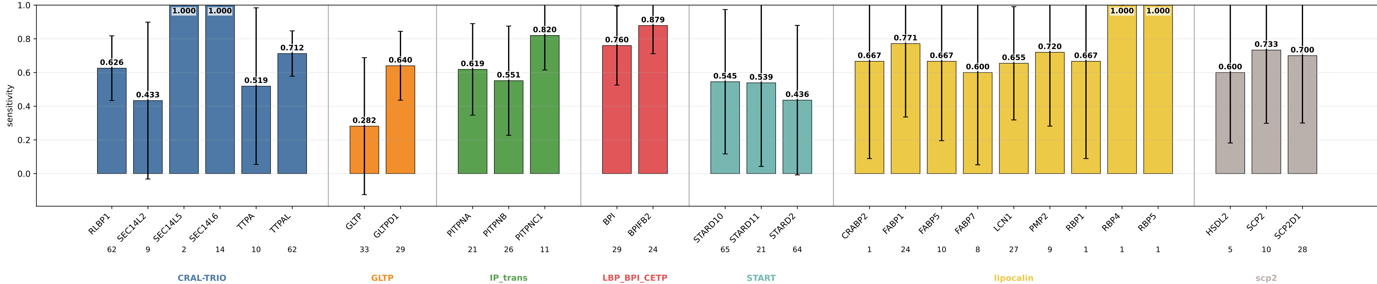
descriptors_no_extent_coarse_add_lipprop_hid4 sensitivity by subgroup descriptors_no_extent_coarse_add_lipprop_hid4 | class weights | lr=0.0001 | weight_decay=0.01 | final_m=4 | final_dropout=0.1 | hiddim=4 | heads=1 | batch=16 | ep=120 | seeds=0,1,2,3,4
