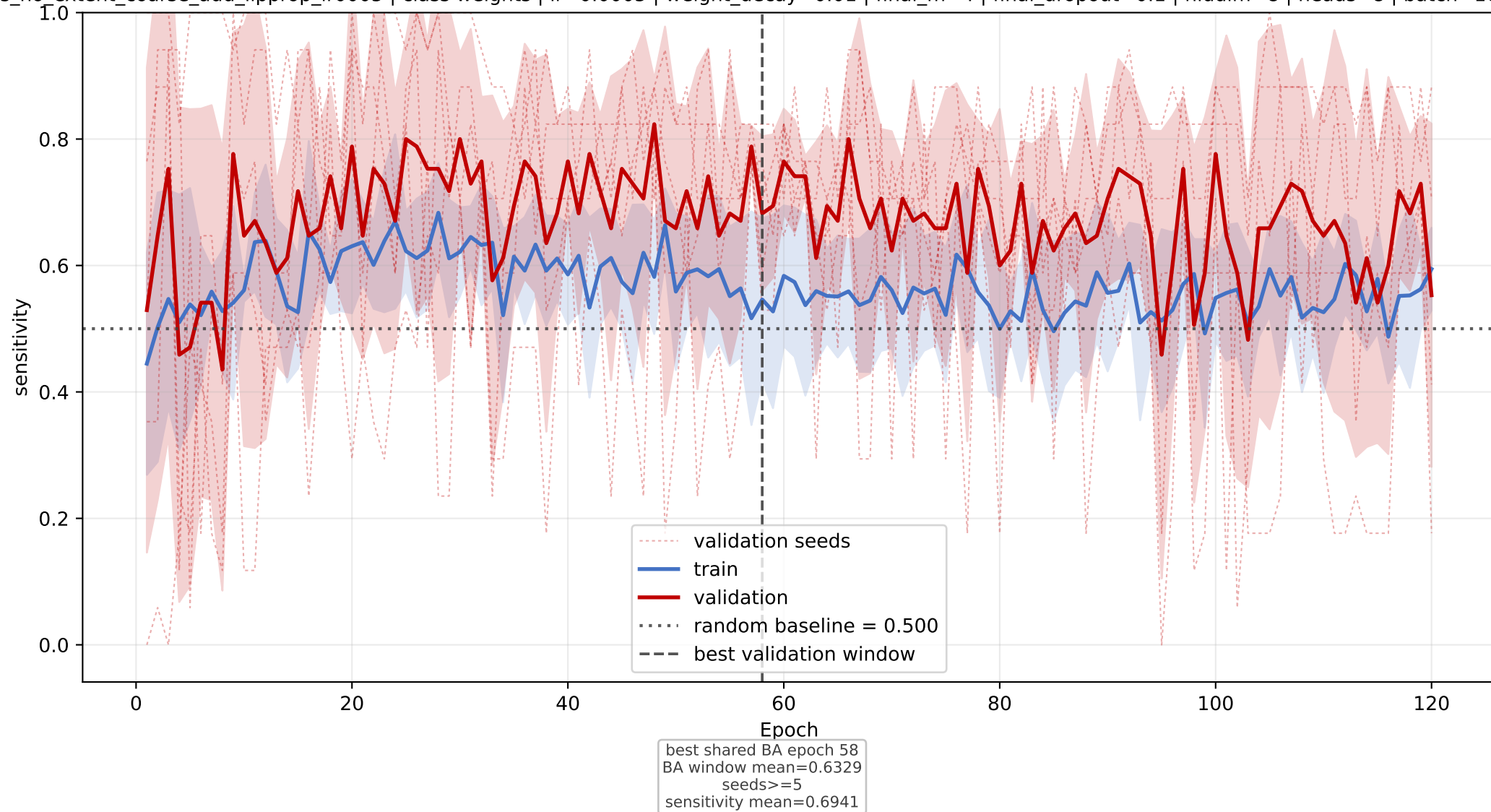
scp2: mean sensitivity learning curve across seeds
