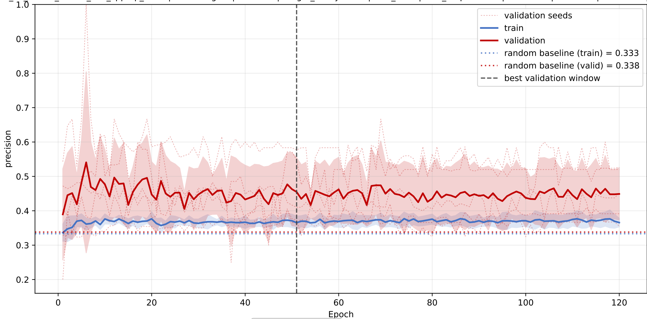
IP_trans: mean precision learning curve across seeds
