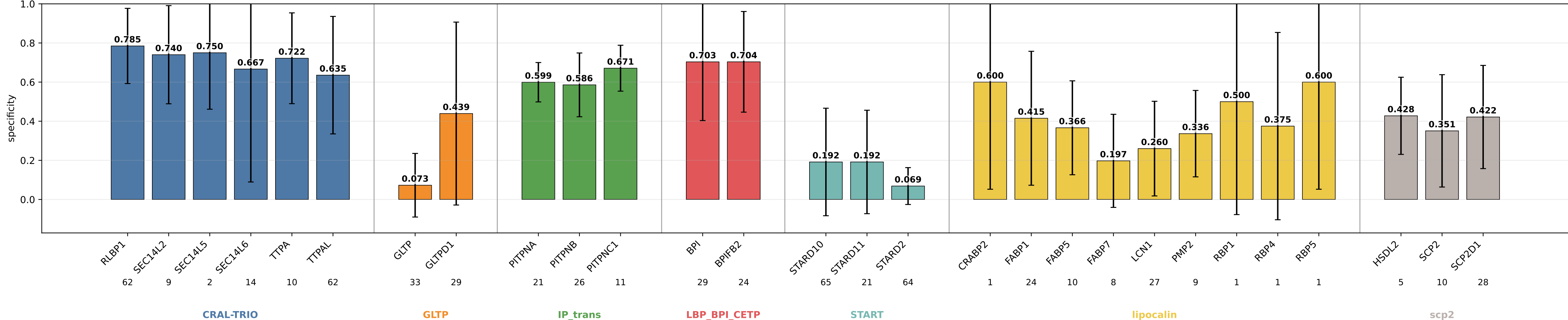
descriptors_no_extent_coarse_add_lipprop_lr005 specificity by subgroup descriptors_no_extent_coarse_add_lipprop_lr005 | class weights | lr=0.005 | weight_decay=0.01 | final_m=4 | final_dropout=0.1 | hiddim=8 | heads=8 | batch=16 | ep=120 | seeds=0,1,2,3,4
