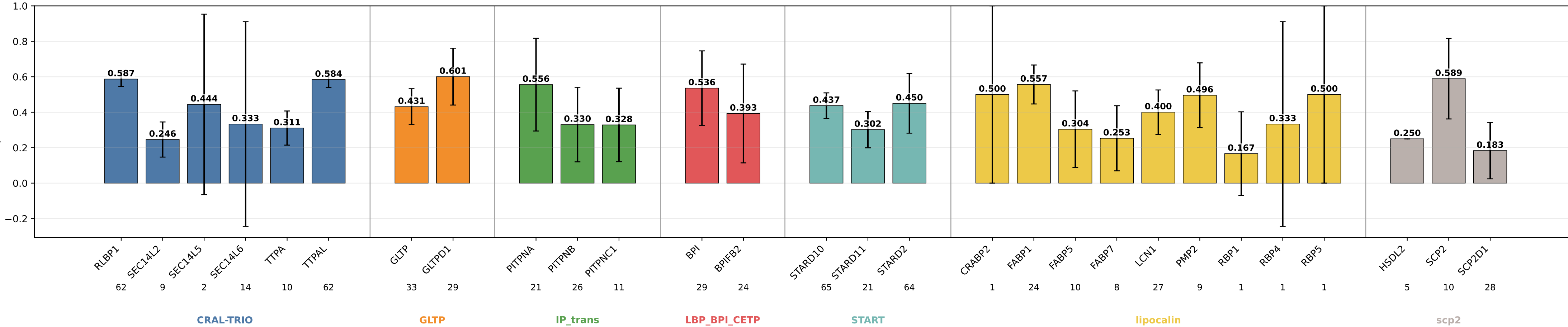
descriptors_no_extent_coarse_add_lipprop_rankprot precision by subgroup descriptors_no_extent_coarse_add_lipprop_rankprot | class weights | lr=0.0001 | weight_decay=0.01 | final_m=4 | final_dropout=0.1 | hiddim=8 | heads=8 | batch=32 | ep=120 | seeds=0,1,2,3,4
