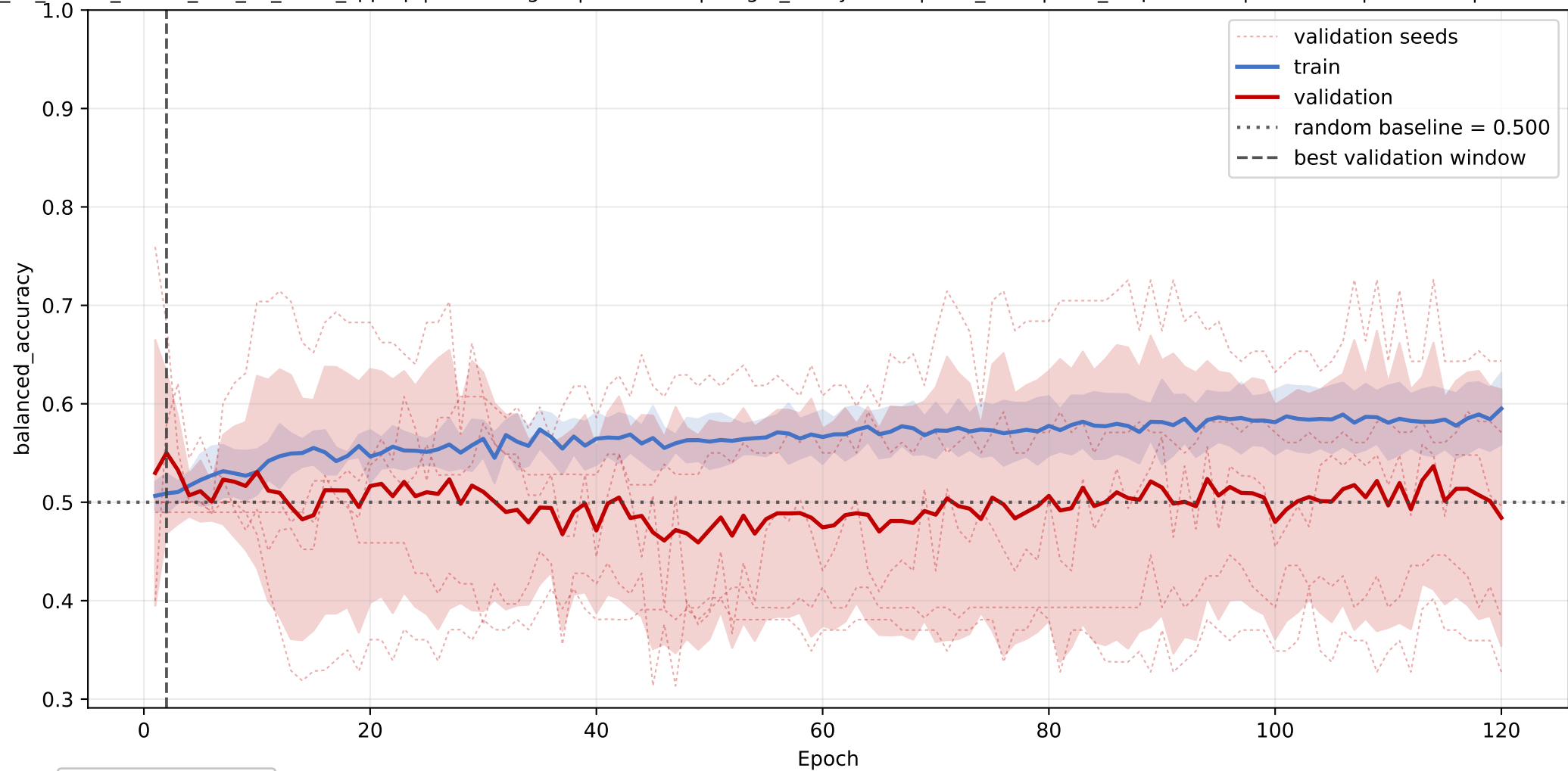
LBP_BPI_CETP: mean balanced_accuracy learning curve across seeds
