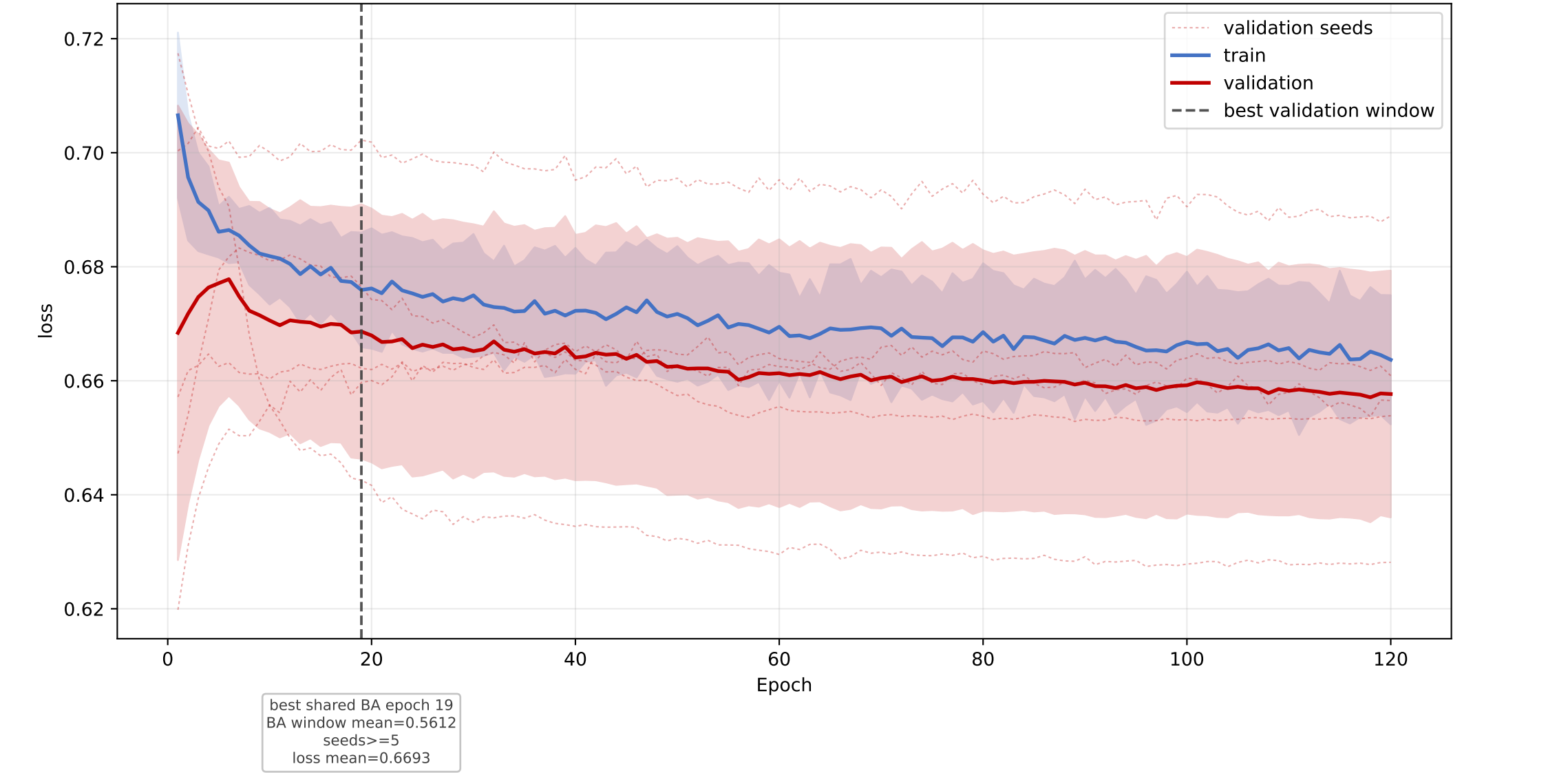
IP_trans: mean loss learning curve across seeds
