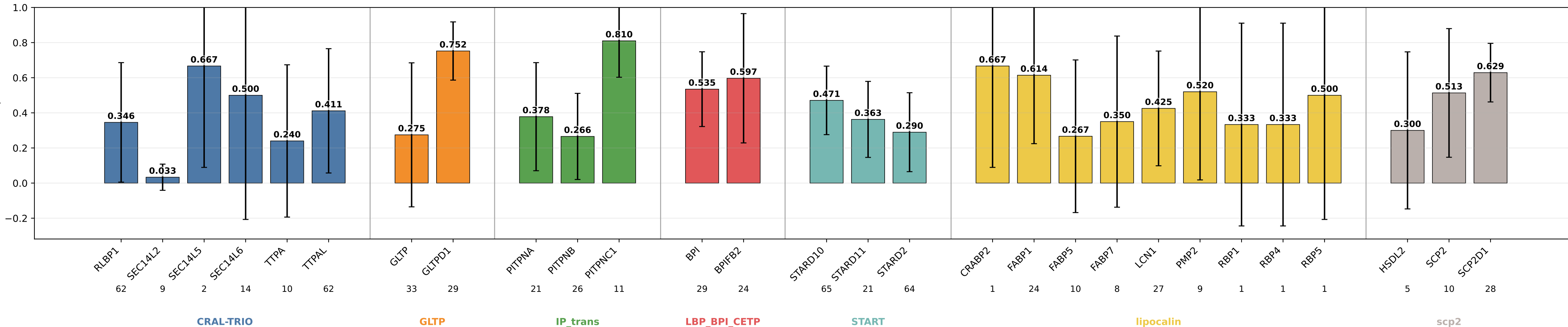
descriptors_no_extent_coarse_flatten sensitivity by subgroup descriptors_no_extent_coarse_flatten | class weights | lr=0.0001 | weight_decay=0.01 | final_m=4 | final_dropout=0.1 | hiddim=8 | heads=8 | batch=16 | ep=120 | seeds=0,1,2,3,4
