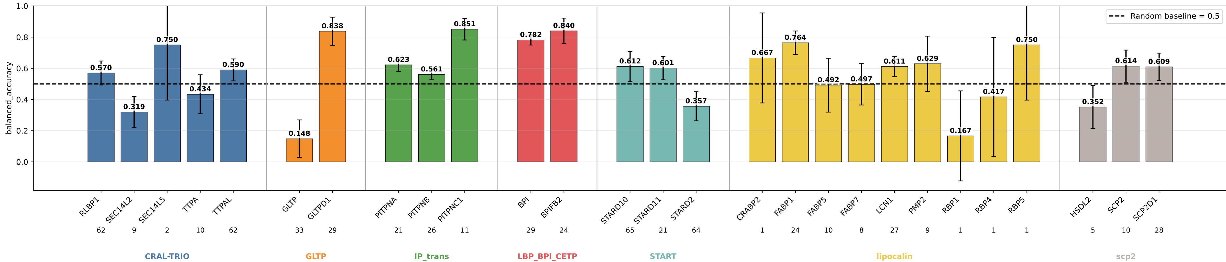
descriptors_no_extent_coarse_pool_add balanced_accuracy by subgroup descriptors_no_extent_coarse_pool_add | class weights | lr=0.0001 | weight_decay=0.01 | final_m=4 | final_dropout=0.1 | hiddim=8 | heads=8 | batch=16 | ep=120 | seeds=0,1,2,3,4
