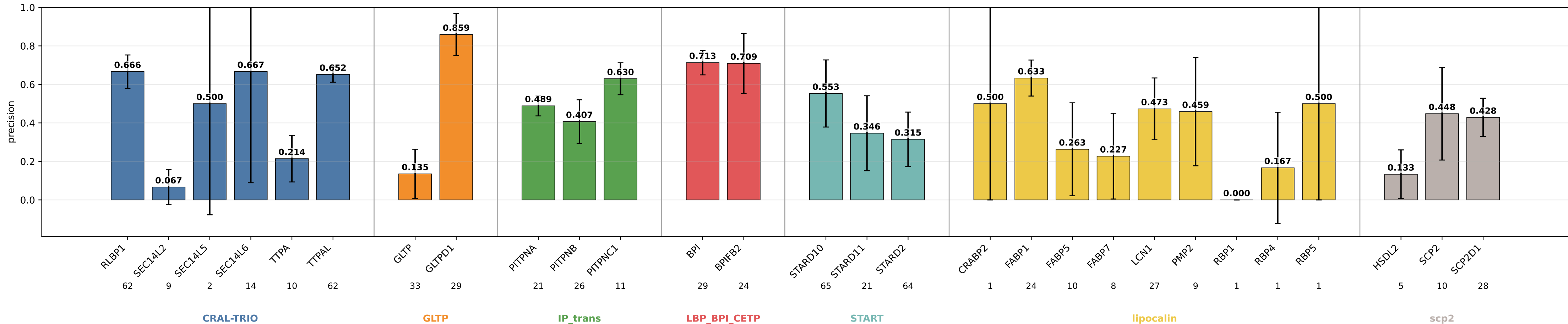
descriptors_no_extent_coarse_pool_add precision by subgroup descriptors_no_extent_coarse_pool_add | class weights | lr=0.0001 | weight_decay=0.01 | final_m=4 | final_dropout=0.1 | hiddim=8 | heads=8 | batch=16 | ep=120 | seeds=0,1,2,3,4
