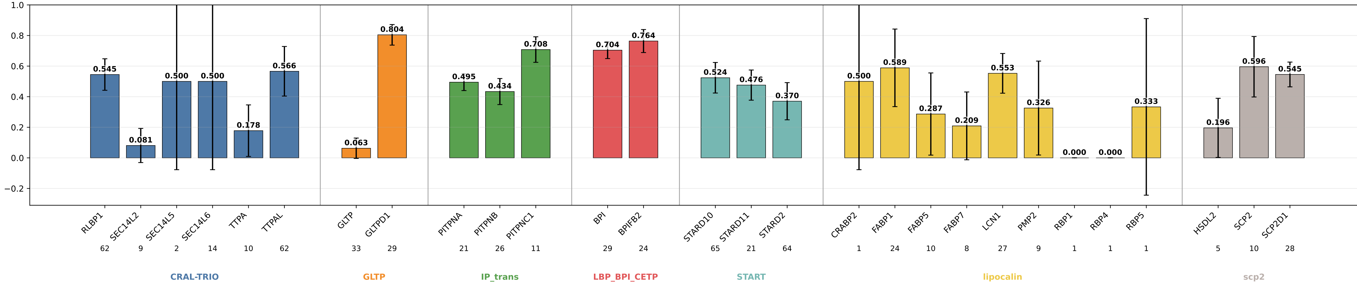
descriptors_no_extnt_coarse_pool_addmax F1 by subgroup descriptors_no_extnt_coarse_pool_addmax | class weights | lr=0.0001 | weight_decay=0.01 | final_m=4 | final_dropout=0.1 | hiddim=8 | heads=8 | batch=16 | ep=120 | seeds=0,1,2,3,4
