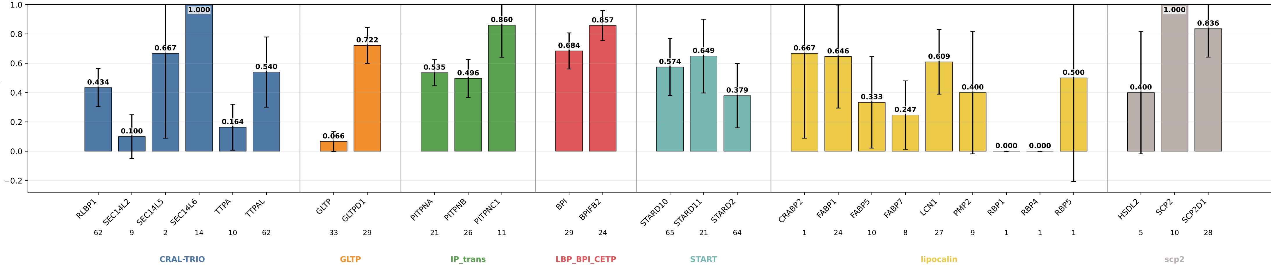
descriptors_no_extent_coarse_pool_addmax sensitivity by subgroup descriptors_no_extent_coarse_pool_addmax | class weights | lr=0.0001 | weight_decay=0.01 | final_m=4 | final_dropout=0.1 | hiddim=8 | heads=8 | batch=16 | ep=120 | seeds=0,1,2,3,4
