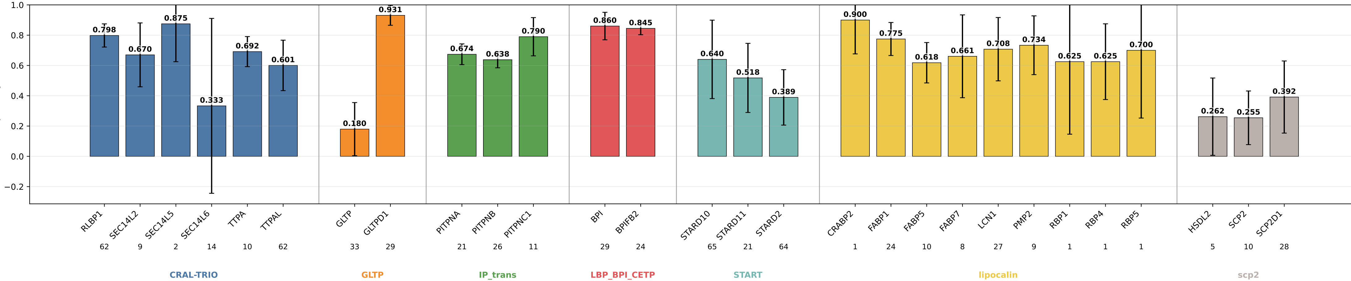
descriptors_no_extent_coarse_pool_addmax specificity by subgroup descriptors_no_extent_coarse_pool_addmax | class weights | lr=0.0001 | weight_decay=0.01 | final_m=4 | final_dropout=0.1 | hiddim=8 | heads=8 | batch=16 | ep=120 | seeds=0,1,2,3,4
