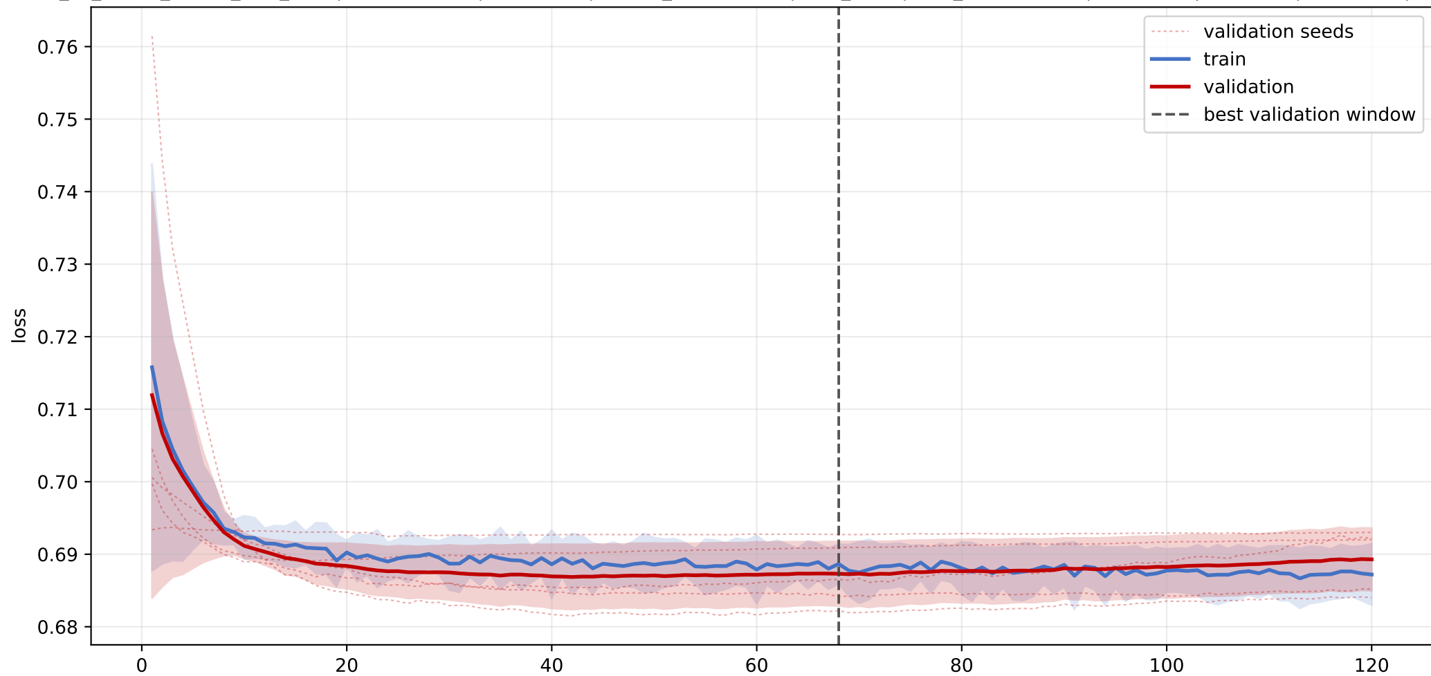
CRAL-TRIO: mean loss learning curve across seeds
