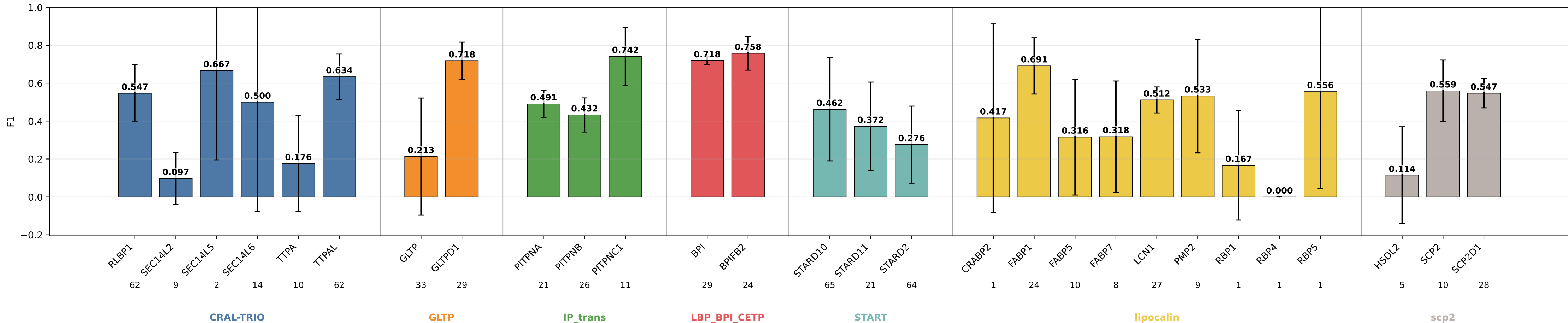
descriptors_no_extent_coarse_pool_gem F1 by subgroup descriptors_no_extent_coarse_pool_gem | class weights | lr=0.0001 | weight_decay=0.01 | final_m=4 | final_dropout=0.1 | hiddim=8 | heads=8 | batch=16 | ep=120 | seeds=0,1,2,3,4
