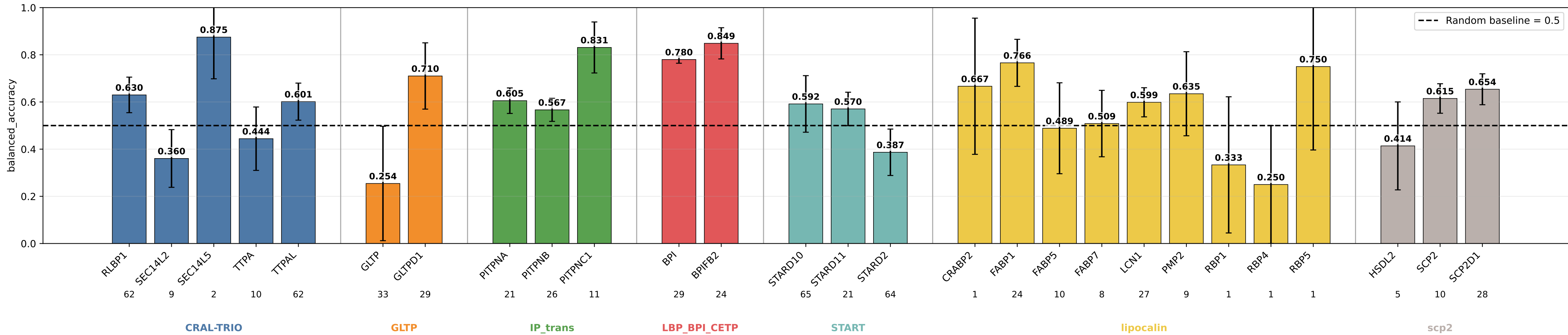
descriptors_no_extent_coarse_pool_gem balanced_accuracy by subgroup descriptors_no_extent_coarse_pool_gem | class weights | lr=0.0001 | weight_decay=0.01 | final_m=4 | final_dropout=0.1 | hiddim=8 | heads=8 | batch=16 | ep=120 | seeds=0,1,2,3,4
