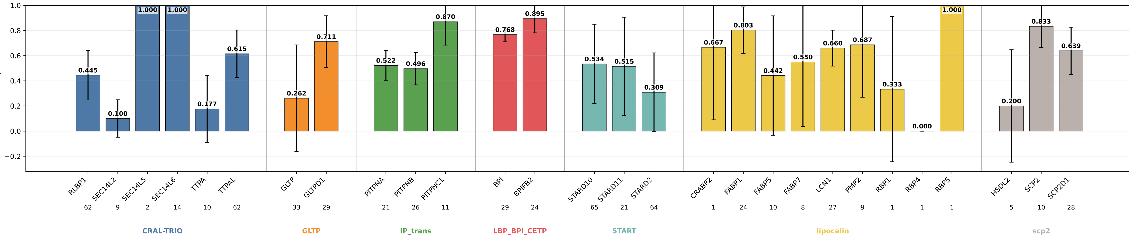
descriptors_no_extent_coarse_pool_gem sensitivity by subgroup descriptors_no_extent_coarse_pool_gem | class weights | lr=0.0001 | weight_decay=0.01 | final_m=4 | final_dropout=0.1 | hiddim=8 | heads=8 | batch=16 | ep=120 | seeds=0,1,2,3,4
