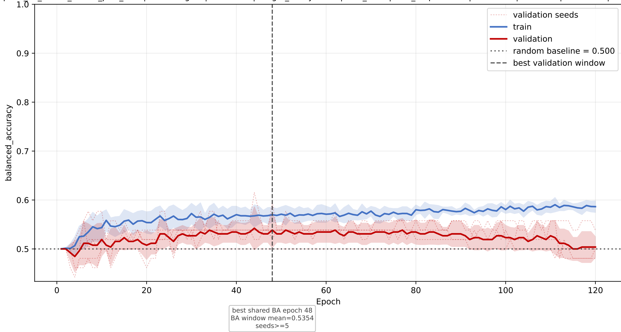
GLTP: mean balanced_accuracy learning curve across seeds
