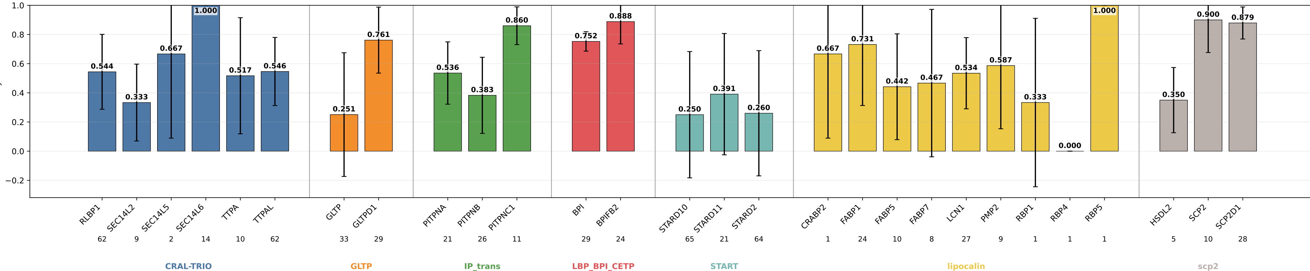
descriptors_no_extent_coarse_pool_max sensitivity by subgroup descriptors_no_extent_coarse_pool_max | class weights | lr=0.0001 | weight_decay=0.01 | final_m=4 | final_dropout=0.1 | hiddim=8 | heads=8 | batch=16 | ep=120 | seeds=0,1,2,3,4
