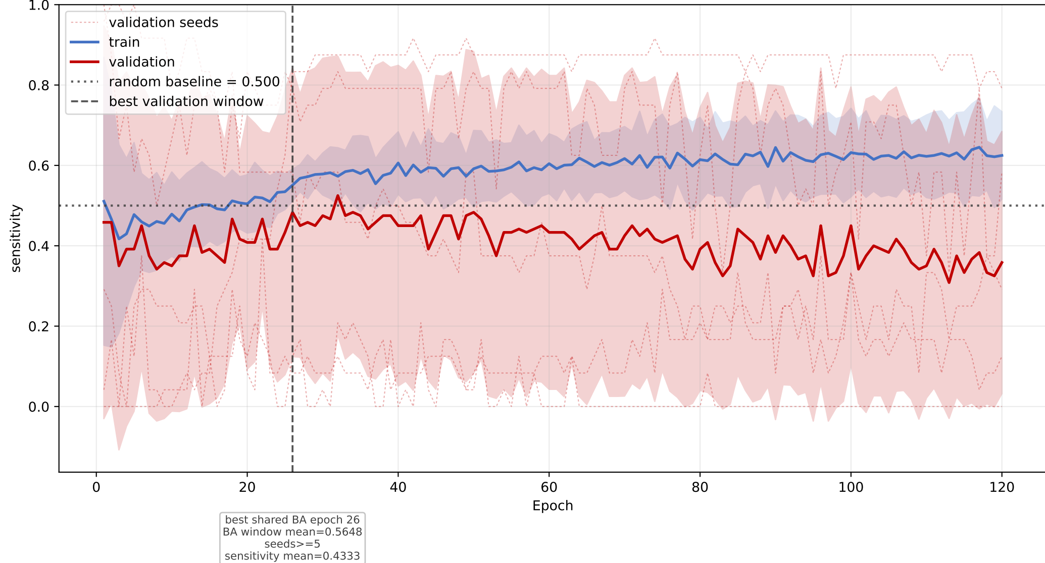
IP_trans: mean sensitivity learning curve across seeds
