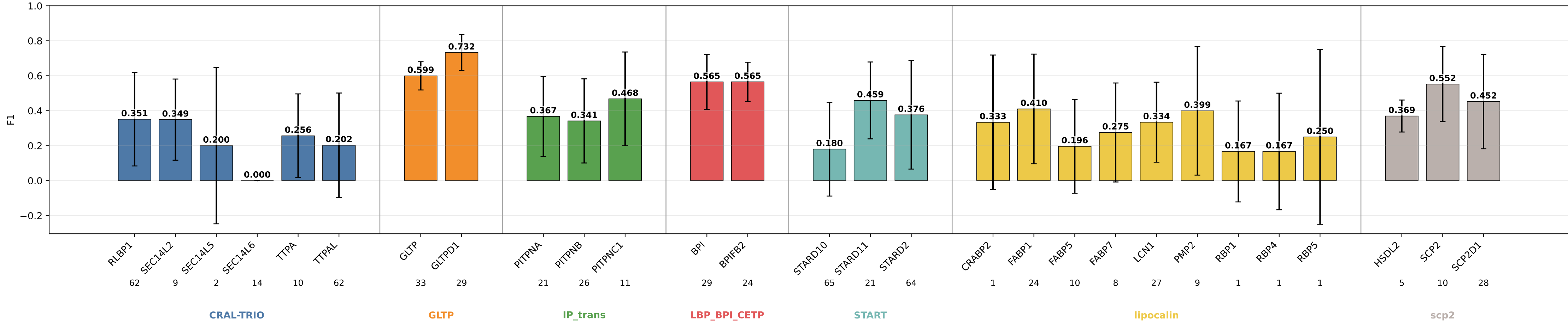
descriptors_pair_only F1 by subgroup descriptors_pair_only | class weights | lr=0.0001 | weight_decay=0.01 | final_m=4 | final_dropout=0.1 | hiddim=8 | heads=8 | batch=16 | ep=120 | seeds=0,1,2,3,4
