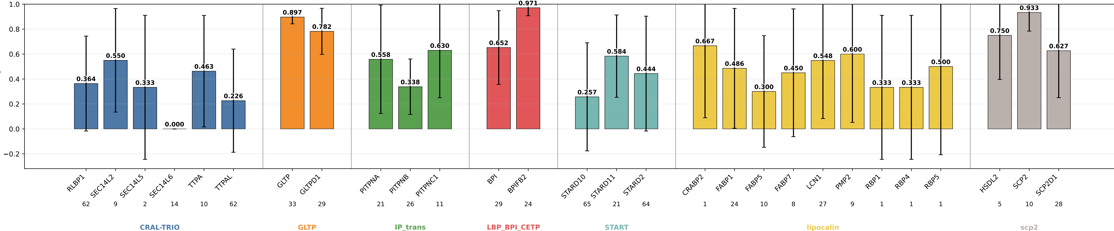
descriptors_pair_only sensitivity by subgroup descriptors_pair_only | class weights | lr=0.0001 | weight_decay=0.01 | final_m=4 | final_dropout=0.1 | hiddim=8 | heads=8 | batch=16 | ep=120 | seeds=0,1,2,3,4
