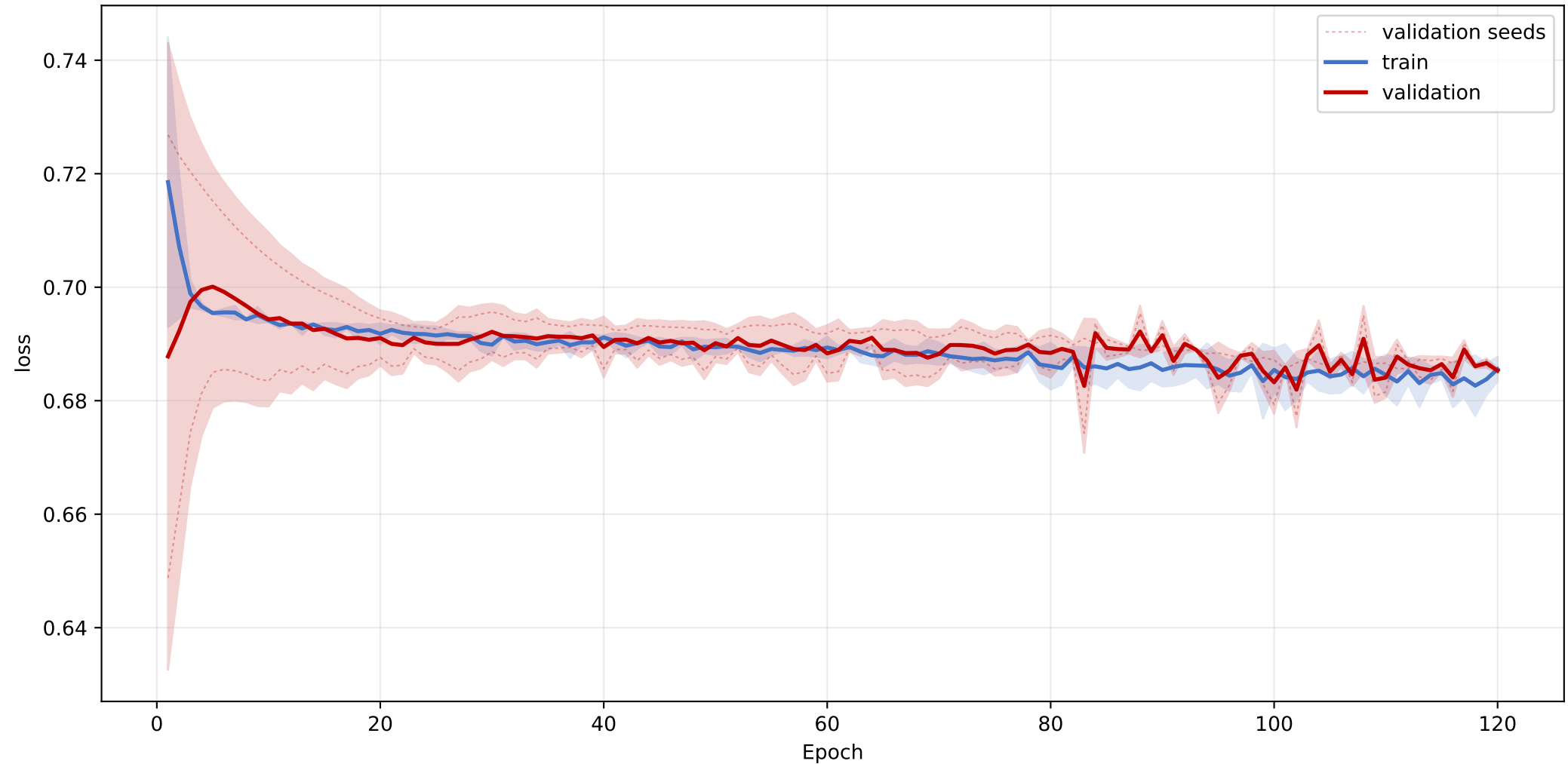
scp2: mean loss learning curve across seeds
